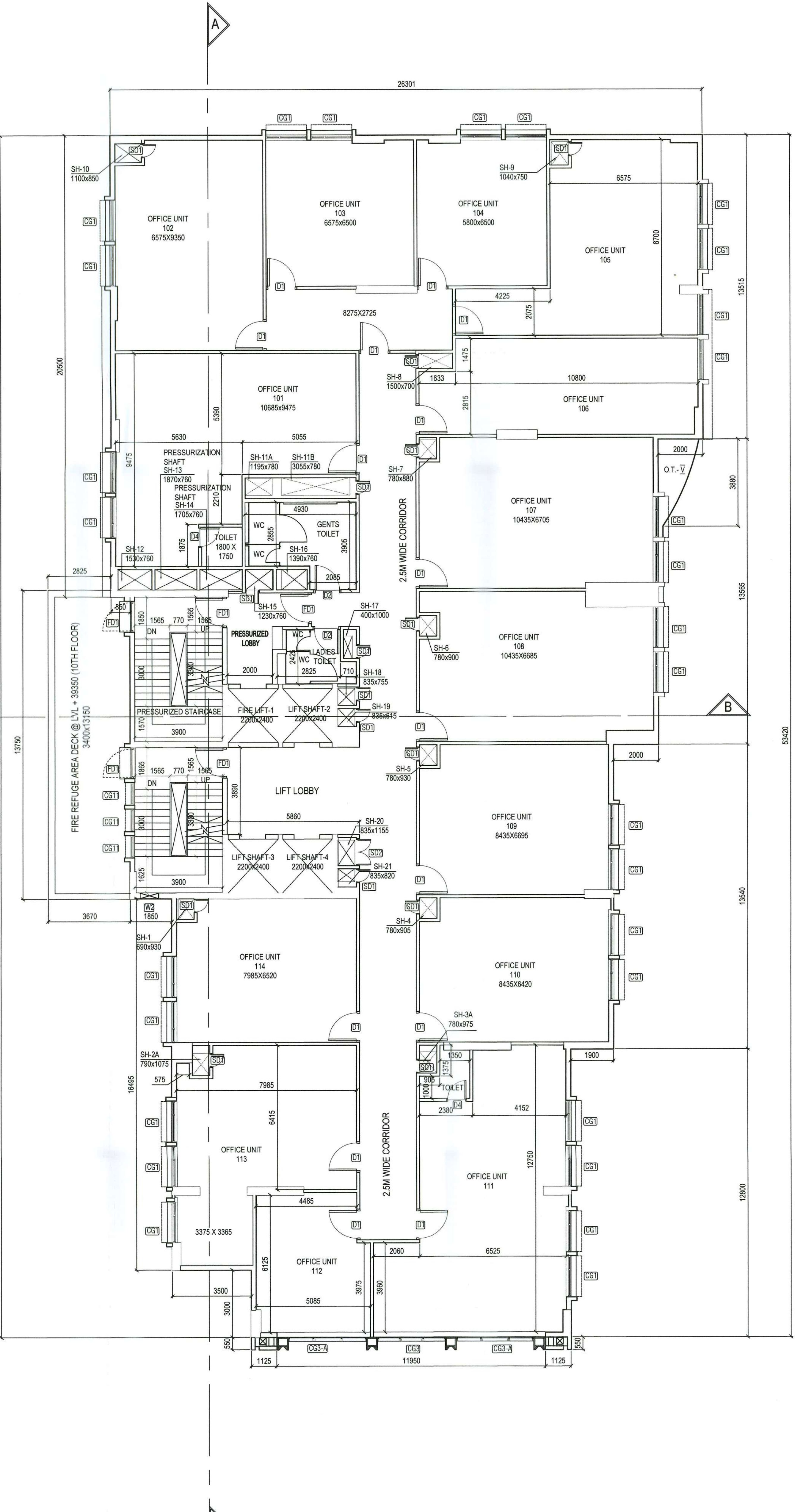
10TH FIRE REFUGE FLOOR LEVEL SCALE - 1 : 100
